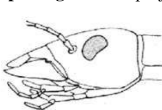
prognathous
