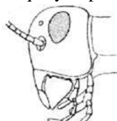
hypognathous
