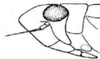
opisthognathous
