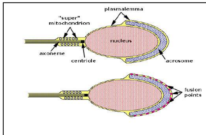
Figure-2: Acrosome reaction
